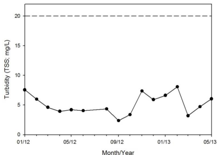
Figure 3 - Plot of Monthly Average Turbidity (TSS) data measured daily in the settlement pond (black dots, solid line); dotted line represents 20mg/L target for treated discharge waters
